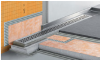
Schluter®-KERDI-LINE Page 144 - 149
